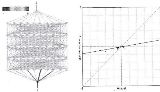
Fig. 10. ANN-BP architecture, the input-output data stream and the predicted data set layout on the regression slope for 4500 [gr].
