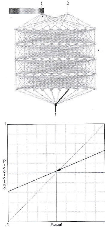
Fig. 7. The ANN-BP architecture, the input-output data stream and the predicted data set layout on the regression slope for 4500 [gr].
