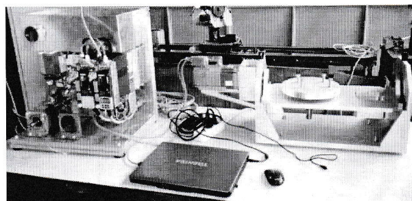
Fig. 1. The experimental system using a rotary table.
