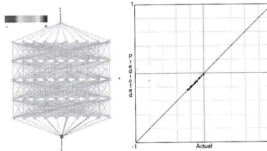
Fig. 9. The ANN-BP architecture, the input-output data stream and the predicted data set layout on the regression slope for 500 [gr].
