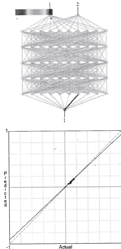
Fig. 6. ANN-BP architecture, the input-output data stream and the predicted data set layout on the regression slope for 500 [gr].
