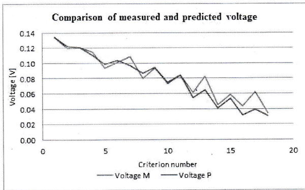
Fig. 3. Comparison of measured and predicted voltage.
