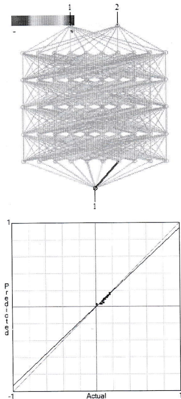
Fig. 5. ANN-BP architecture, the input-output data stream and the predicted data set layout on the regression slope for 0 [gr].
