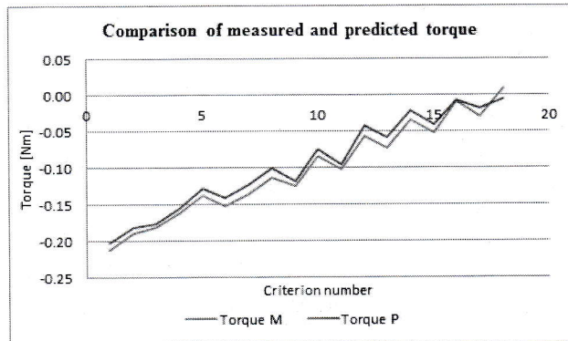
Fig. 4. Comparison of measured and predicted torque.
