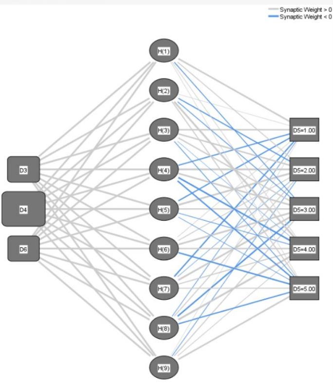
Figure 2. RBF architecture.
